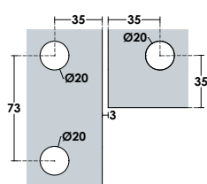
Glass Cut
