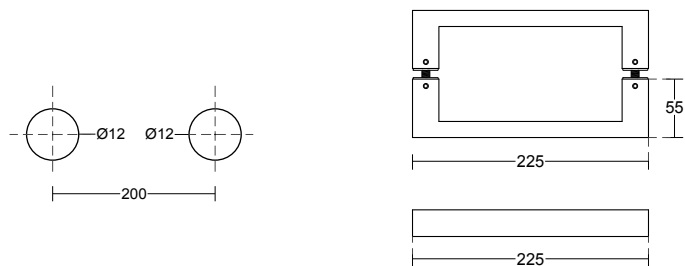
Glass Cut
