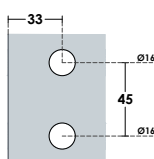
Glass Cut
