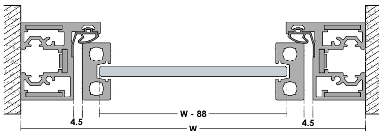
GT12 Frame | GT14 Door Section Details
