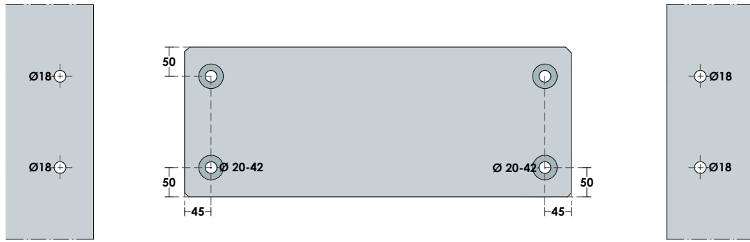
Glass Preparation
