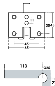
Glass Cut
