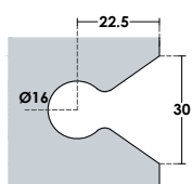
Glass Cut
