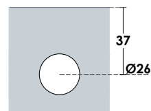
Glass Cut
