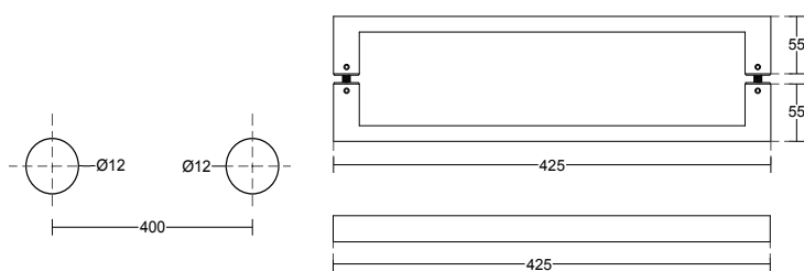
Glass Cut
