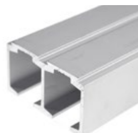
PCA-GT05 Guide Track Profile 580 cm | Length 1,802kg | Weight/meter Aluminium | Material Natural Anodize, Satin | Finish
