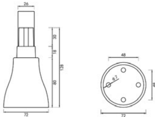
POST Dimensions
