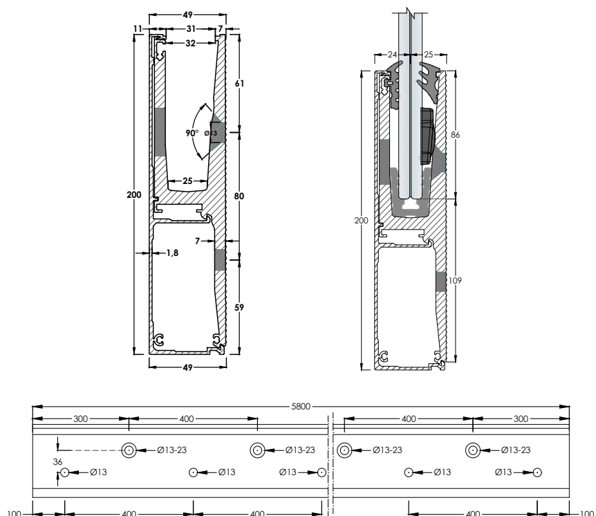
Profile Holes
