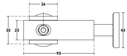
PCA-FC11 Glass Staircase Fitting 560 gr | Weight 50kg | Max Weight 16-30mm | Glass Thickness Stainless Steel 304 | Material Satin | Finish
