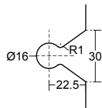
Glass Cut
